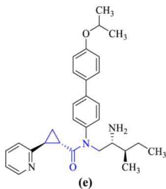
GPR88 agonist cAMP regulation EC 50 = 77 nM(GPR88)
