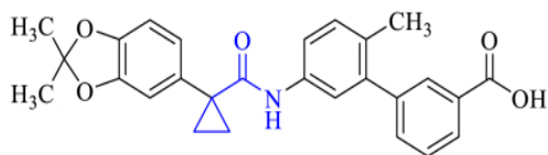
(b) Lumacaftor (To treat certain type of Cystic fibrosis)
