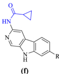
Harmine scaffold (Anti-Inflammatory)
