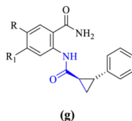
Anti proliferative and Cytotoxicity activity scaffolds
